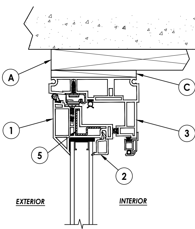
3 VERTICAL CROSS SECTION 3 Shown w/ 1x sub-buck option
