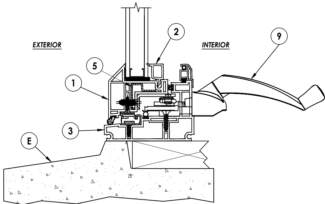
1 VERTICAL CROSS SECTION 3 Optional masonry sill
